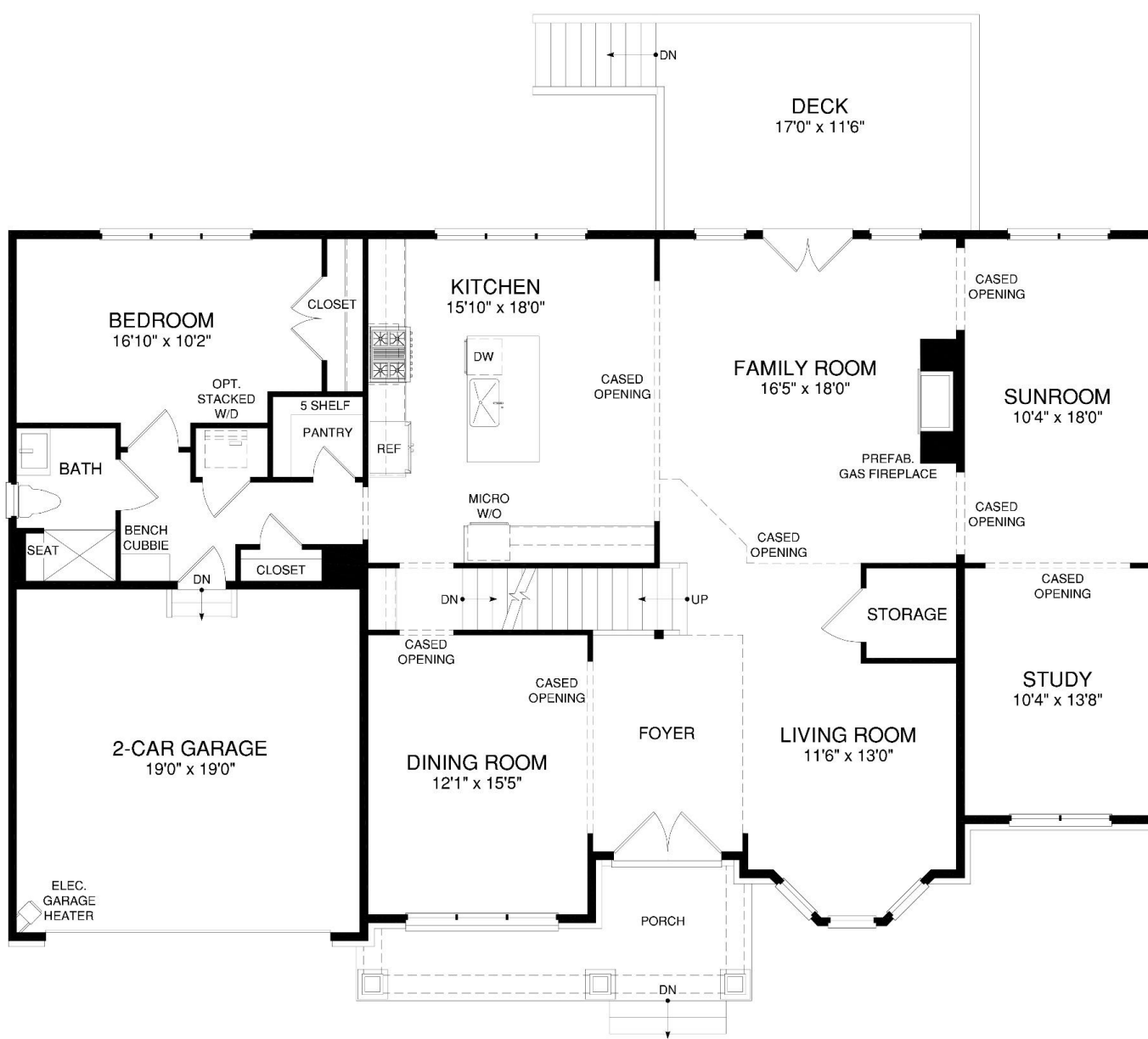
BARTLETT – MAIN LEVEL PLAN
