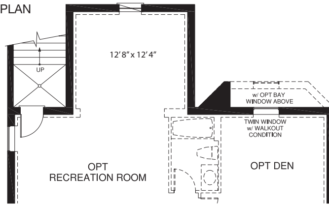
PARTIAL BASEMENT w/ OPT MORNING ROOM
