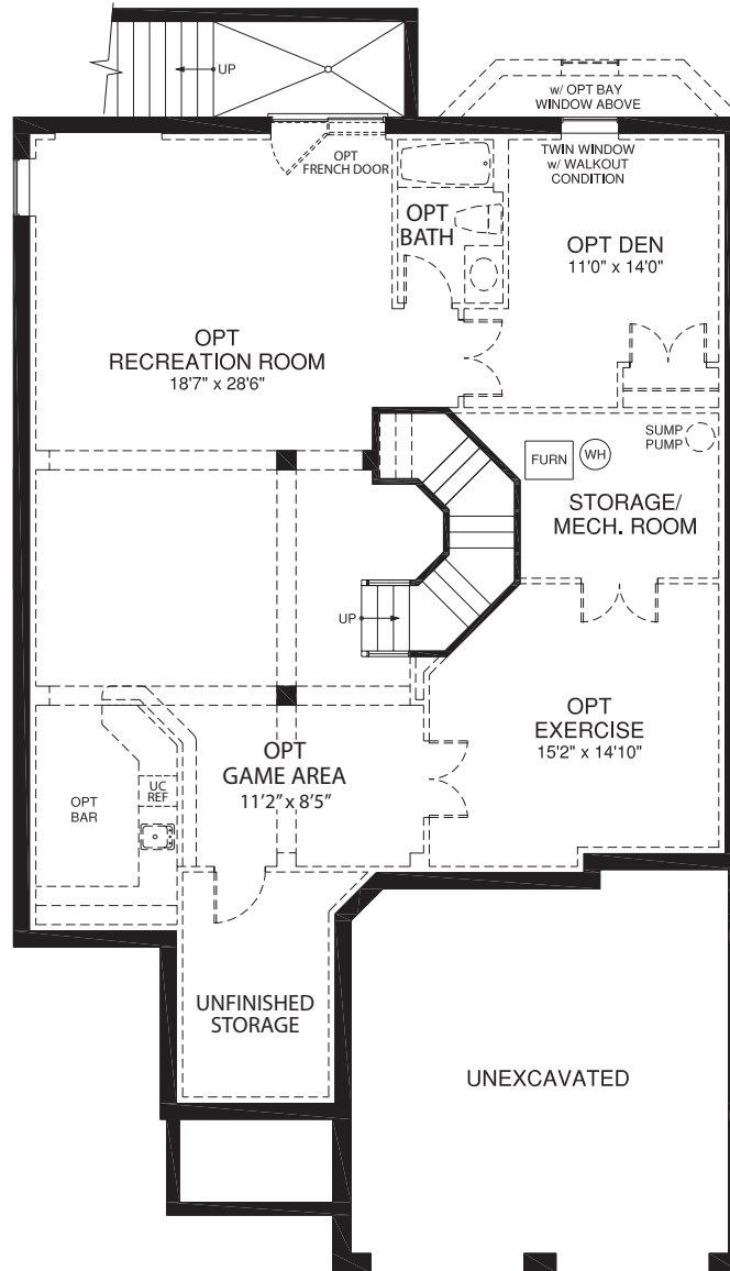
BASEMENT PLAN w/ ELEV. #1 & #2
