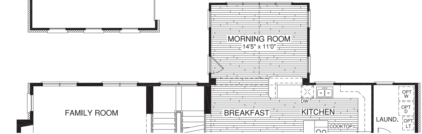
PARTIAL FIRST FLOOR w/ OPT MORNING ROOM
